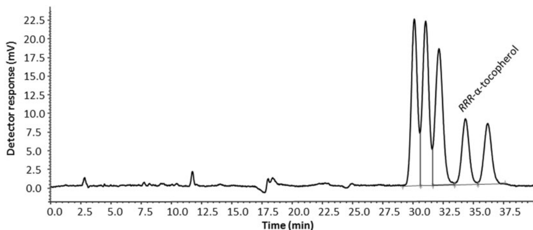
Figure 2. Chromatogram of all-rac- \alpha -tocopherol standard (1 µg/mL) illustrating baseline separation of RRR- \alpha -tocopherol from the seven other stereoisomers (peak area ratio = 2:2:2:1:1, 0 dec.pl.); mobile phase = isooctane–ethanol–propan-2-ol (100:0.06:0.06, v/v/v), flow rate = 1.0 mL/min, fluorescence \lambda_{\text{ex}} = 292 nm, \lambda_{\text{em}} = 330 nm, column oven 50 °C.
