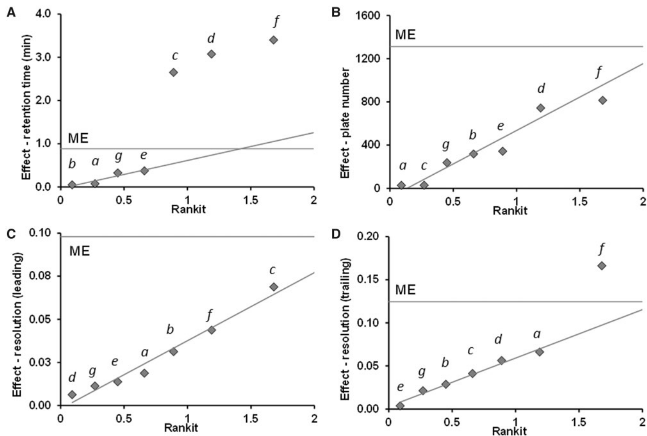
Figure 4. Half-normal plots for chromatographic robustness: (A) retention time, (B) theoretical plate number, (C) resolution of RRR- \alpha -tocopherol peak with preceding peak, (D) resolution of trailing peak with RRR- \alpha -tocopherol peak; a = environmental temperature, b = mobile phase moisture, c = polar modifier, d = flow rate, e = injection volume, f = column oven temperature, g = dummy factor, ME = margin of error.
