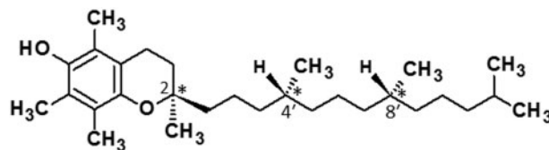
Figure 1. Structure of RRR- \alpha -tocopherol (chiral centers marked with * located on carbons 2, 4', and 8').
