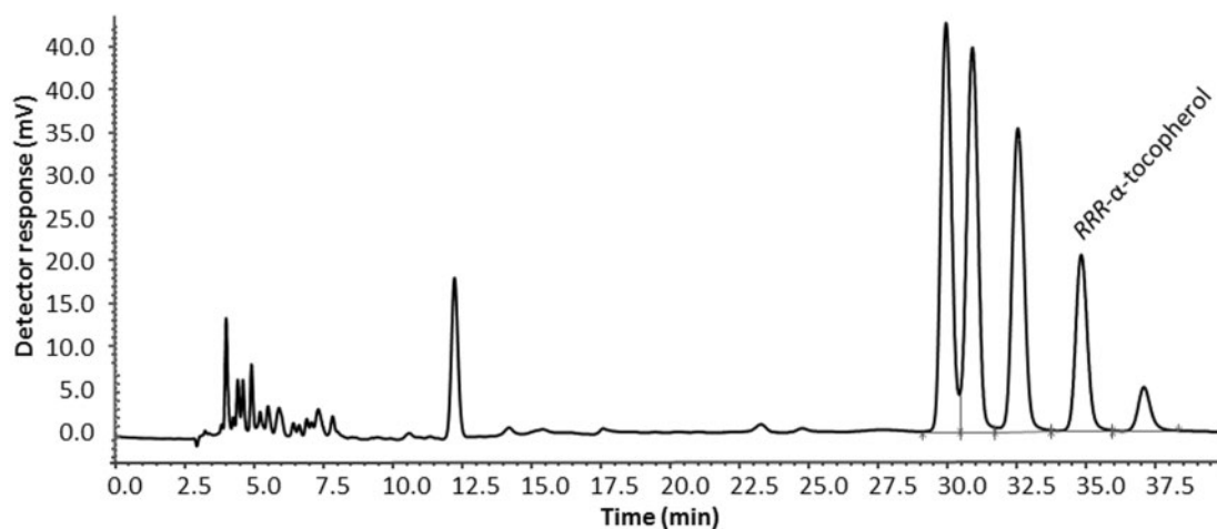
Figure 3. Chromatogram of infant formula sample illustrating baseline separation of RRR- \alpha -tocopherol from the seven other stereoisomers; mobile phase = isooctane-ethanol-propan-2-ol (100:0.06:0.06, v/v/v), flow rate = 1.0 mL/min, fluorescence \lambda_{\text{ex}} = 292 nm, \lambda_{\text{em}} = 330 nm, column oven 50 °C.
