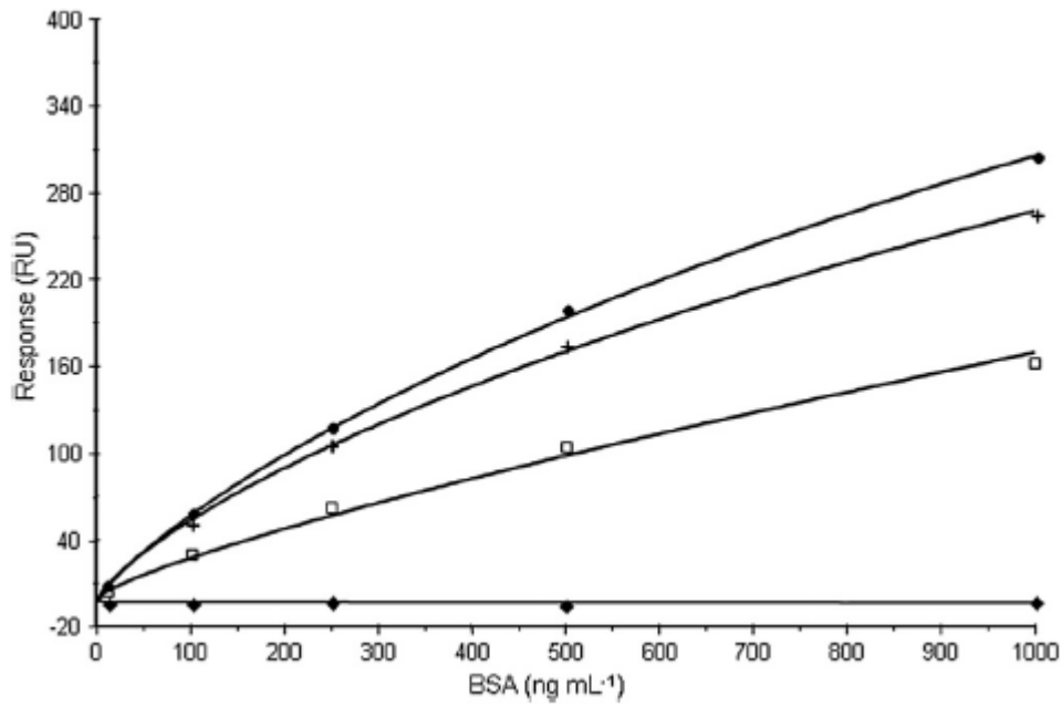
Figure 2. Binding response (RU) of BSA injected over four independent anti-BSA immobilised flow cells under direct assay conditions: (+) rabbit (Sigma); (●) sheep (Bethyl); (□) rabbit (Bethyl); (◆) goat (Santa Cruz)
