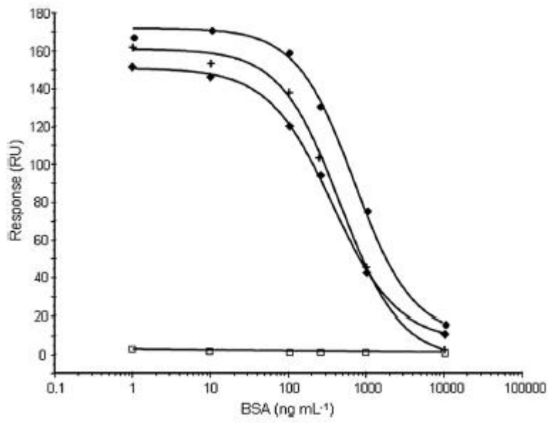
Figure 1. Binding response (RU) of polyclonal anti-BSA antibodies injected over a single BSA-immobilised sensor surface under inhibition assay conditions: (●) rabbit (Sigma, 2.5 µg mL -1 ); (+) sheep (Bethyl, 1.0 µg mL -1 ); (◆) rabbit (Bethyl, 1.0 µg mL -1 ); (□) goat (Santa Cruz, 5.0 µg mL -1 )
