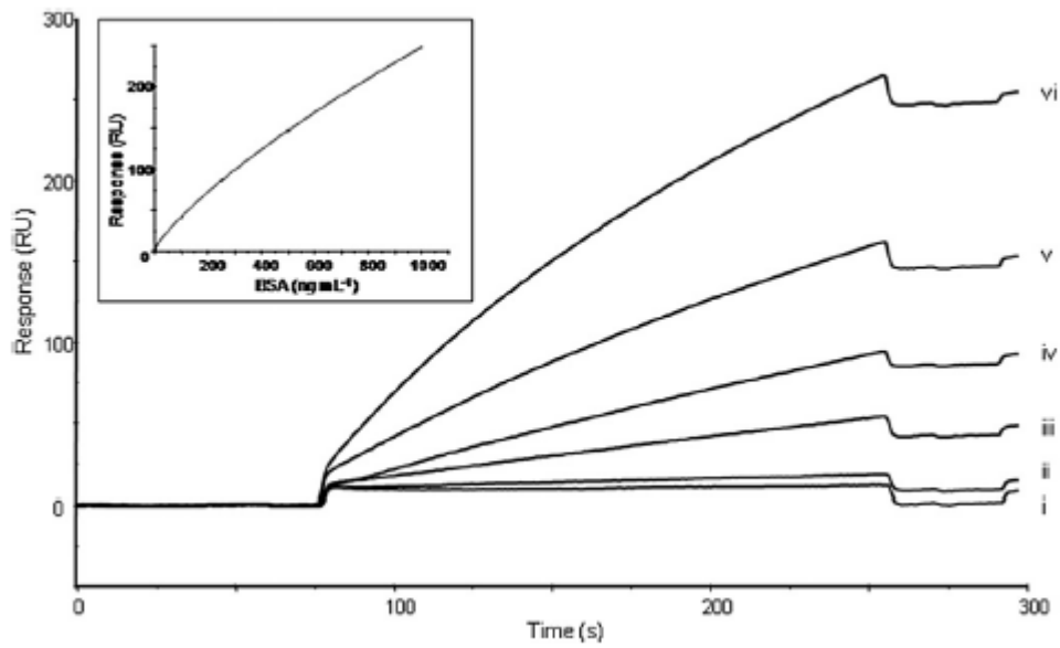
Figure 3. Overlaid sensorgrams obtained for the concentration series of BSA at (i) 0 ng mL -1 , (ii) 10 ng mL -1 , (iii) 100 ng mL -1 , (iv) 250 ng mL -1 , (v) 500 ng mL -1 , and (vi) 1000 ng mL -1 , under optimised direct assay conditions (regeneration phase of each cycle removed for clarity). Inset: dose-response calibration derived from relative binding response (RU)
