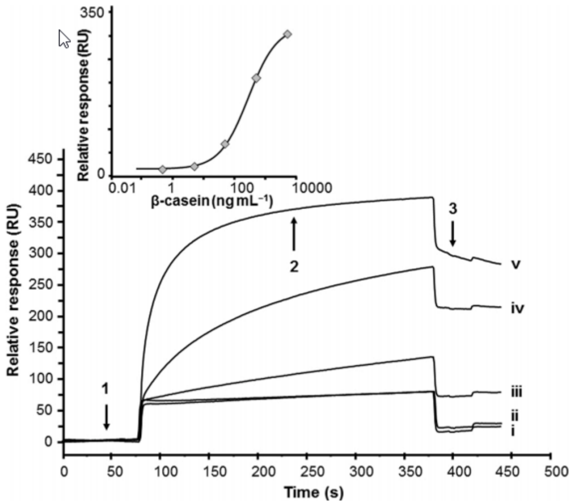
Fig. 2 . Superimposed sensorgrams for \beta -casein calibration standards [(i) 0 ng mL -1 , (ii) 5.5 ng mL -1 , (iii) 55 ng mL -1 , (iv) 550 ng mL -1 , (v) 5500 ng mL -1 ], in singlicate, over an anti- \beta -casein antibody immobilised surface under direct assay conditions (regeneration phase of each cycle removed for clarity): 1, baseline; 2, association; 3, binding level. Inset: derived dose-response calibration curve
