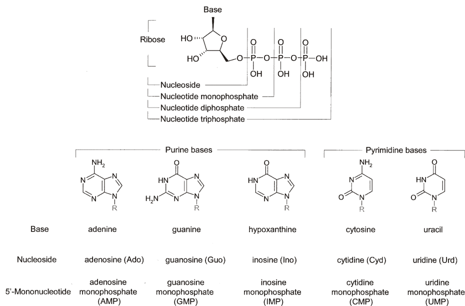
Figure 1. Structural relationship between nucleotides, nucleosides, and nucleobases.
